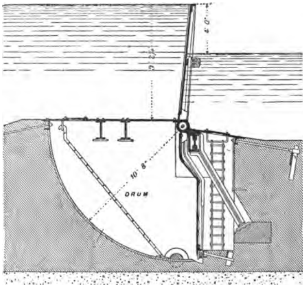
DRUM WEIR ON THE SPREE AT CHARLOTTENBURG.
